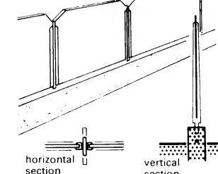
㉔ Partition fence of ornamental wired glass on concrete base
